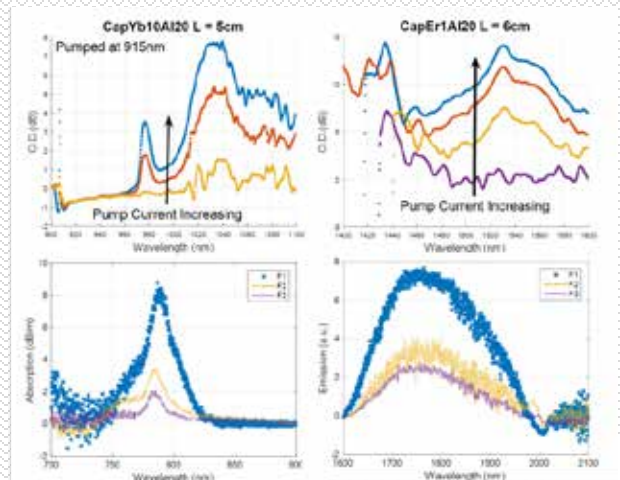
Spectral responses of fabricated fibers
